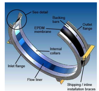
Flexible Connections
